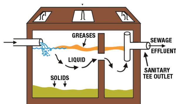
Two-Compartment Septic System
